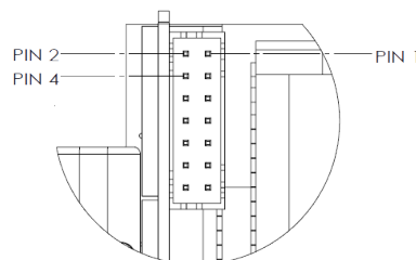
J400 Pin map
