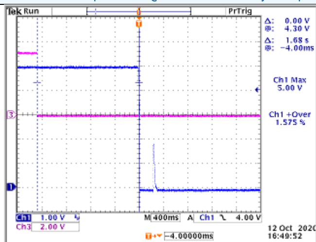
Hold-up Time Test @100Vac/60Hz - Standby 5V output
