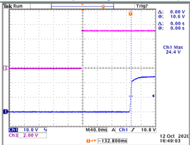
Turn-on Delay Time Test @115Vac/60Hz - Main output
