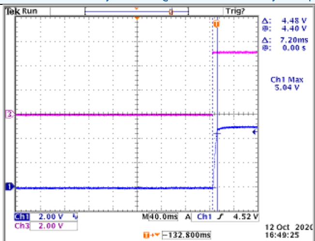
Turn-on Delay Time Test @115Vac/60Hz - Standby 5V output
