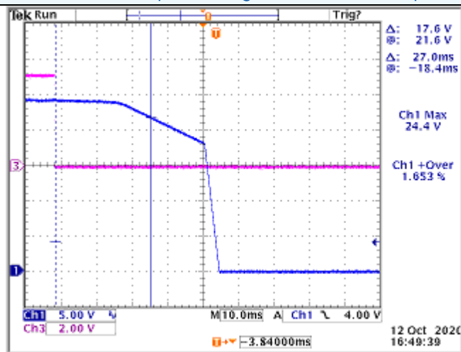
Hold-up Time Test @100Vac/60Hz - Main output
